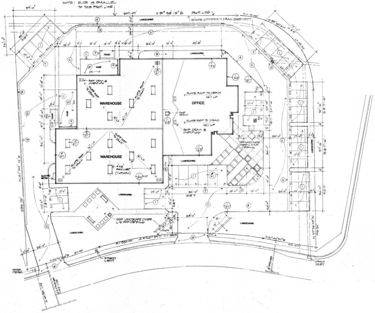
SITE PLAN
